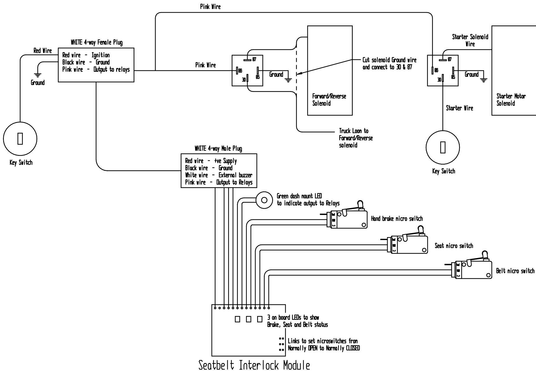
Seatbelt Interlock Wiring
